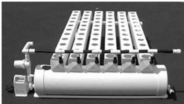
Figure 9.7- This is an example of an aeroponics system.
