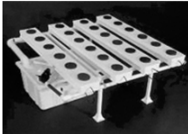
Figure 9.4 - This is a picture of an NFT system.
